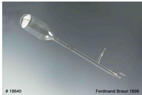
# 18640 Ferdinand Braun 1898 Museum Baruther Glashütte / Turowski [CC BY-NC-SA]
